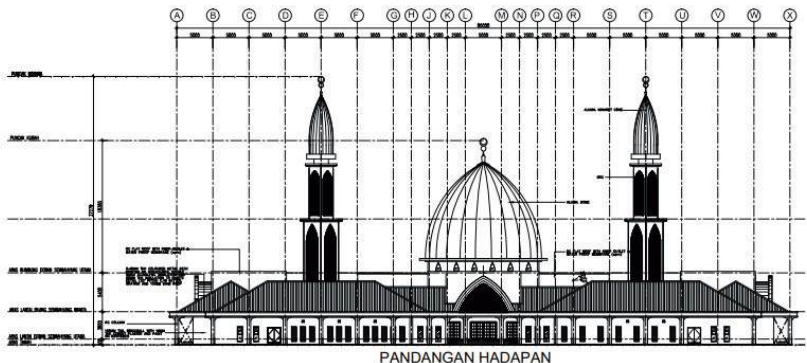
PANDANGAN HADAPAN
